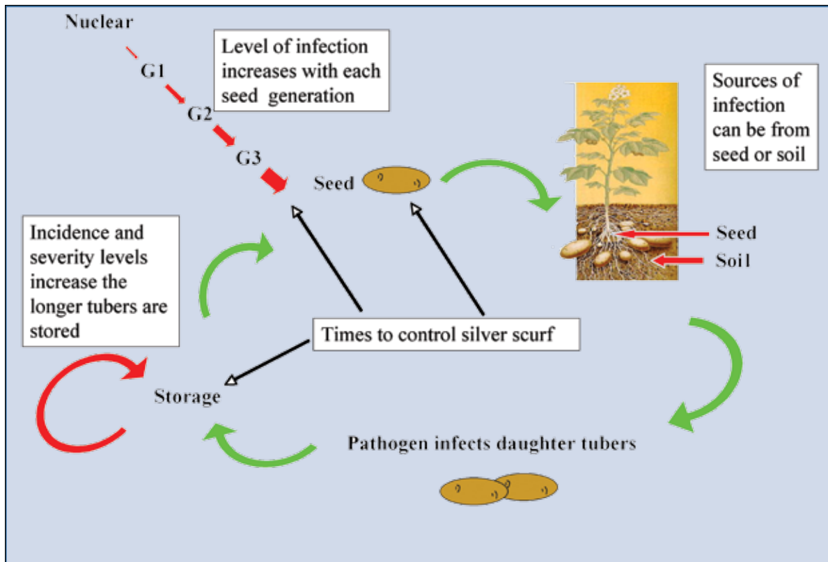
Figure 7.—Silver scurf disease cycle (modified from Brad Geary, Brigham Young University).
